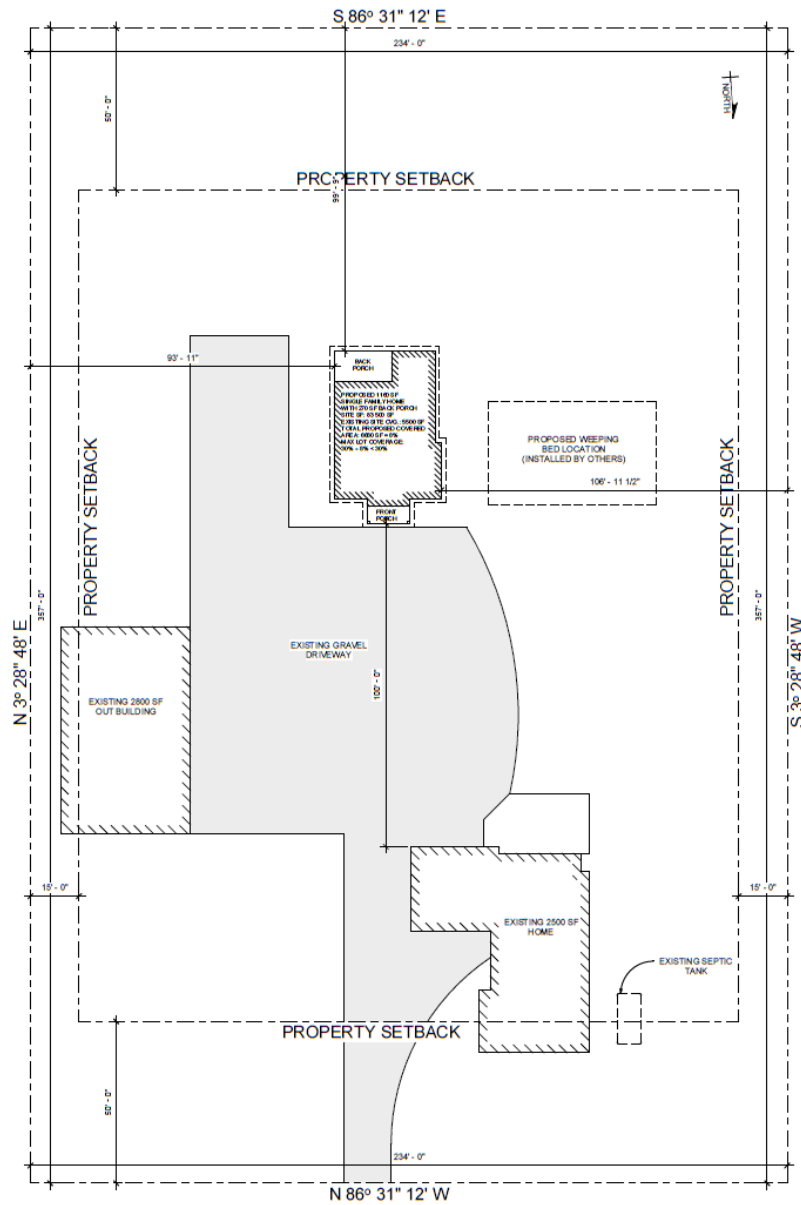
SITE PLAN SCALE: 1/4" = 1' - 0"
