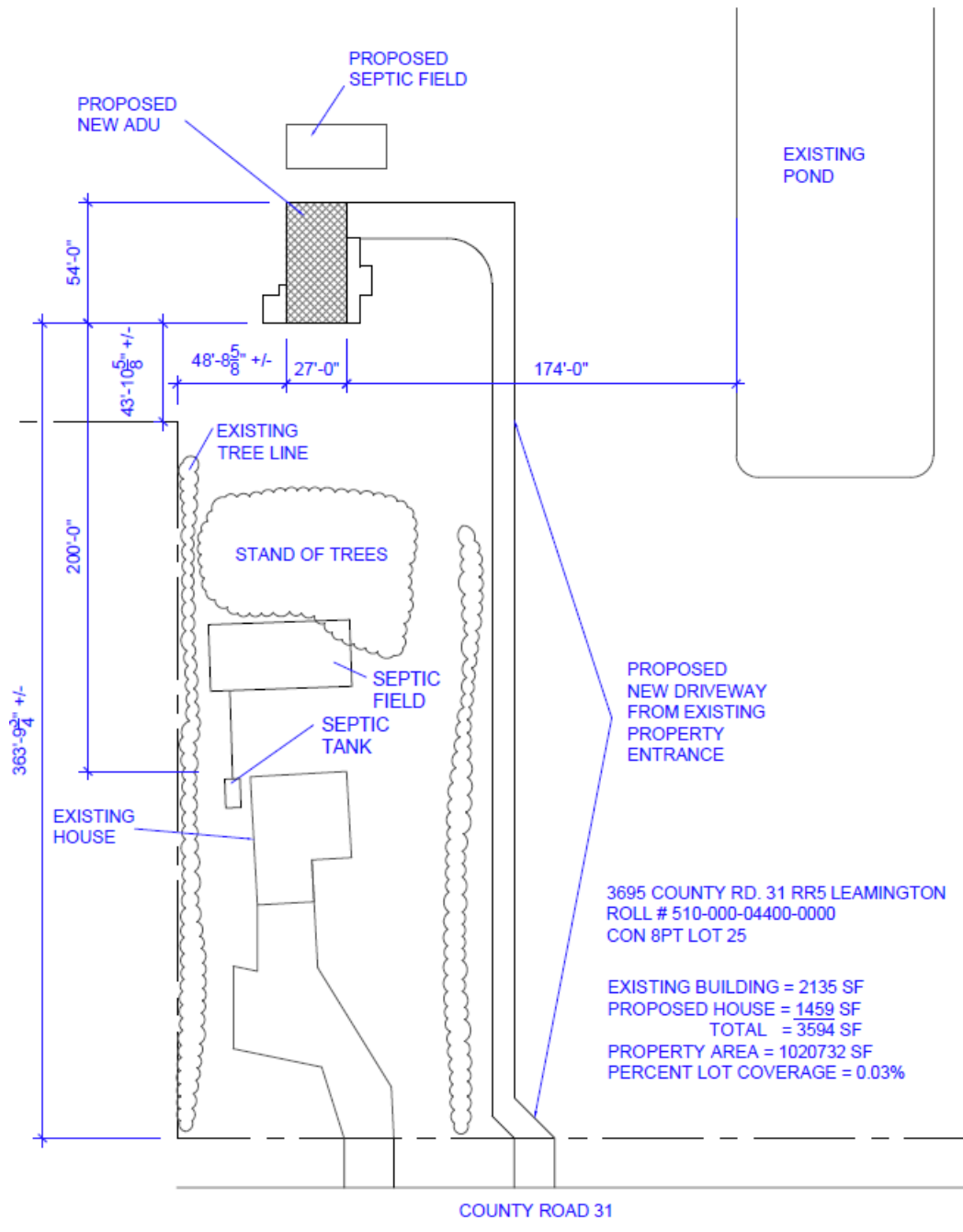
SITE PLAN 1" = 60 0'
